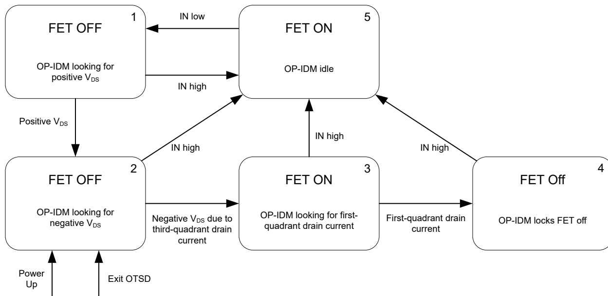
9-6. Operational Ideal-Diode Mode (OP-IDM) State Machine
