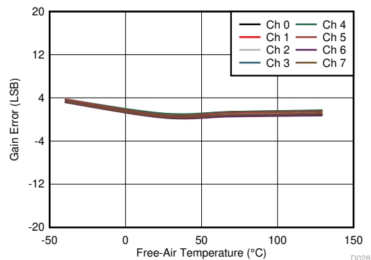
FIG 6-31. Gain Error vs Free-Air Temperature (±10 V, Across Channels)
