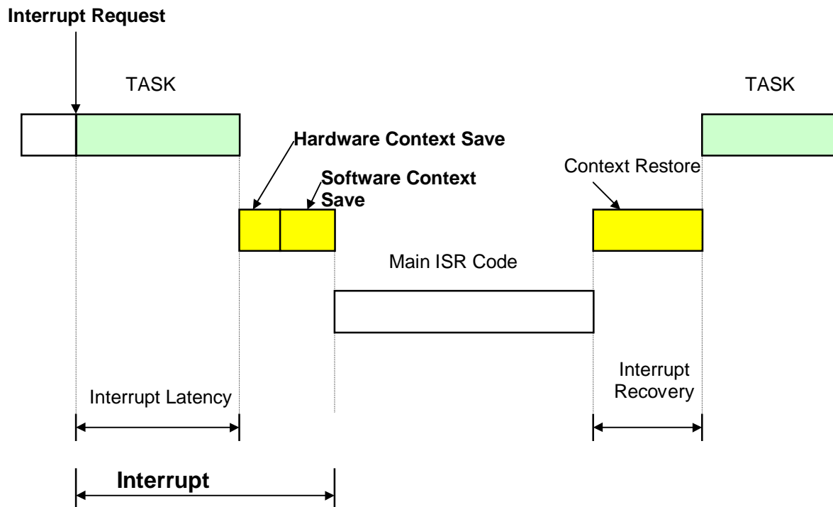
Figure 2. Interrupt Latency, Response, and Recovery Time
